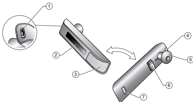
Figure 2: Jabra GO headset as seen from the outer and inner sides, respectively
