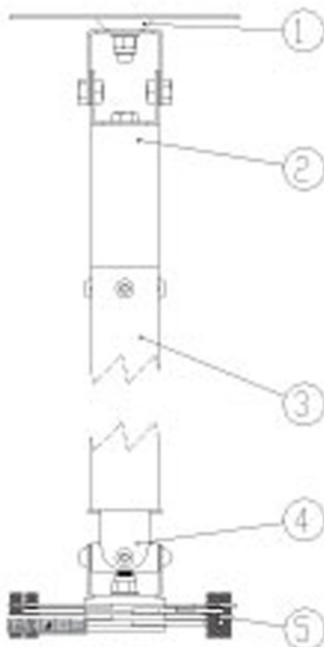
Sloping Ceiling configuration
