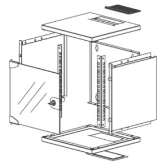
EXPLODED VIEW
